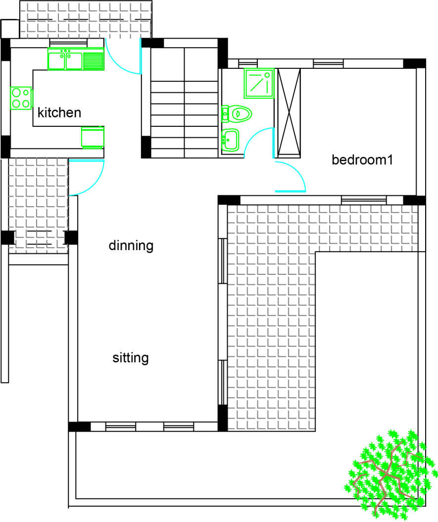
Ground Floor
